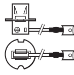
PK22s IEC 7004-47
